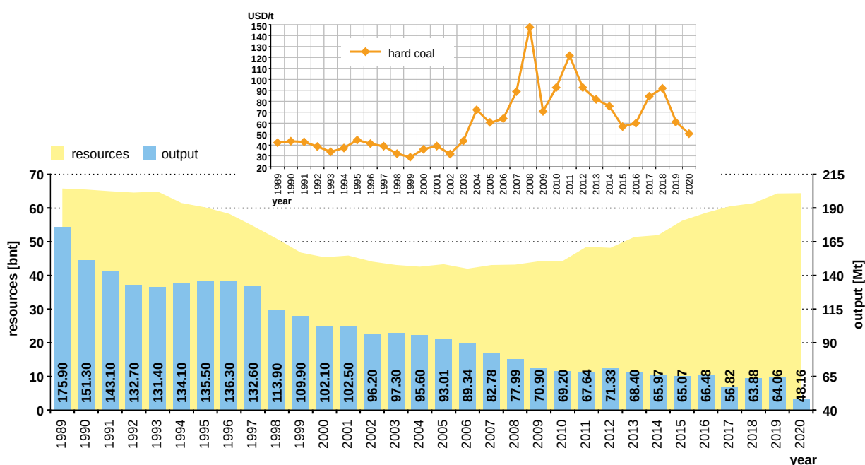
Figure 8.4.1. Hard coal anticipated economic resources, output and annual prices in 1989–2020 (steam coal, Northwest Europe marker price)
